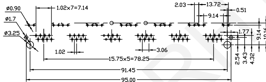
PCB Layout
